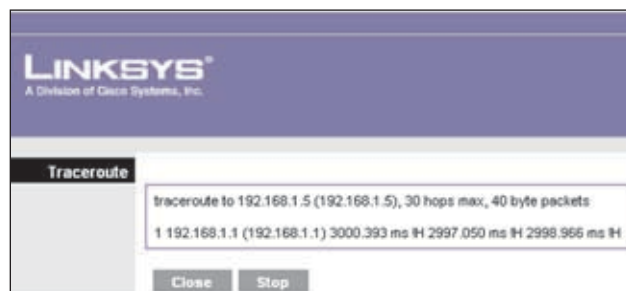
Diagnostics > Traceroute
